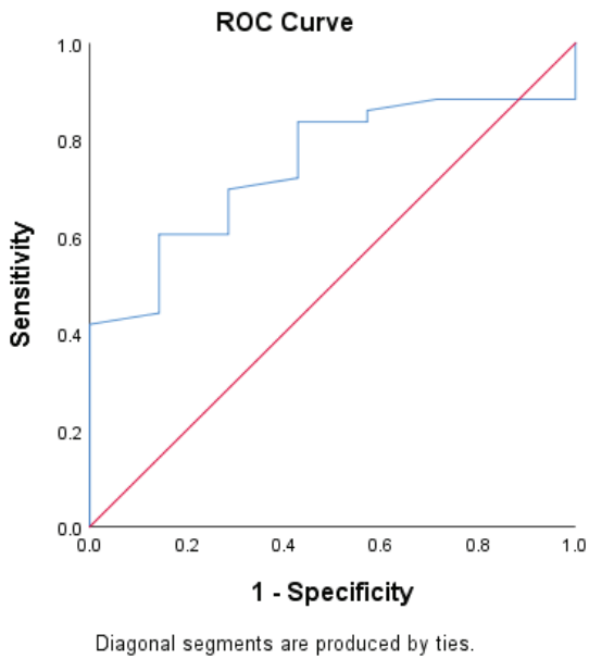
Figure 1: ROC Analysis.
